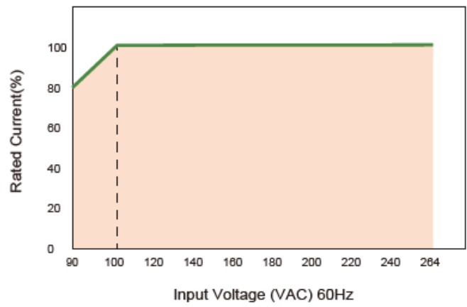
Static Characteristics
